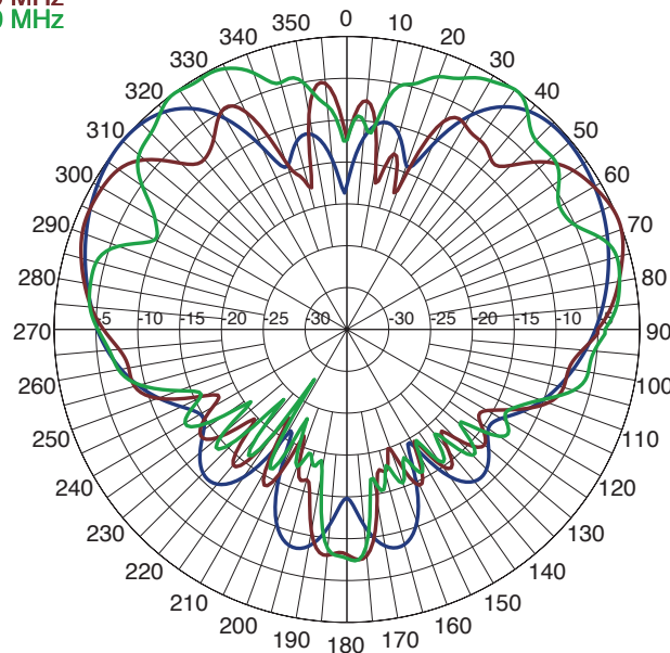
BMLPVMB/LTE - Elevation
