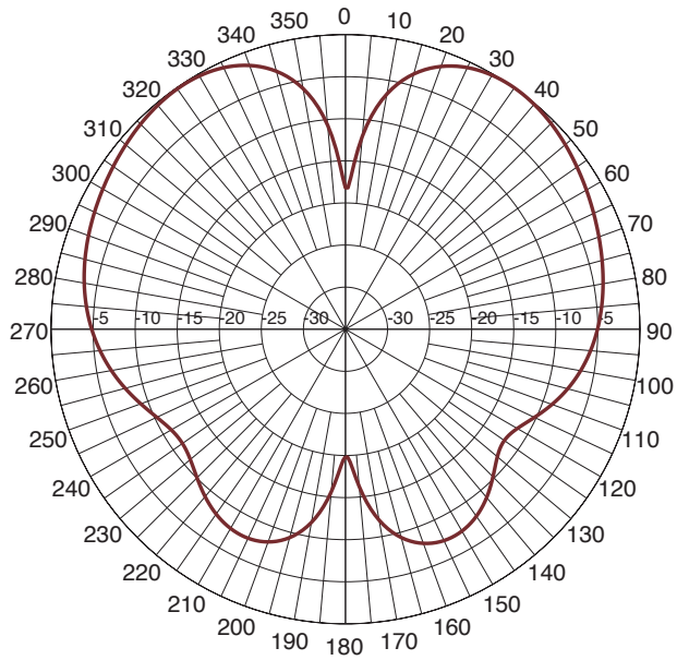
MLPV430 - Elevation
