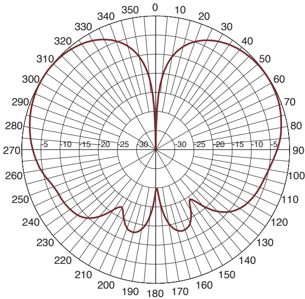
MLPV800 - Elevation
